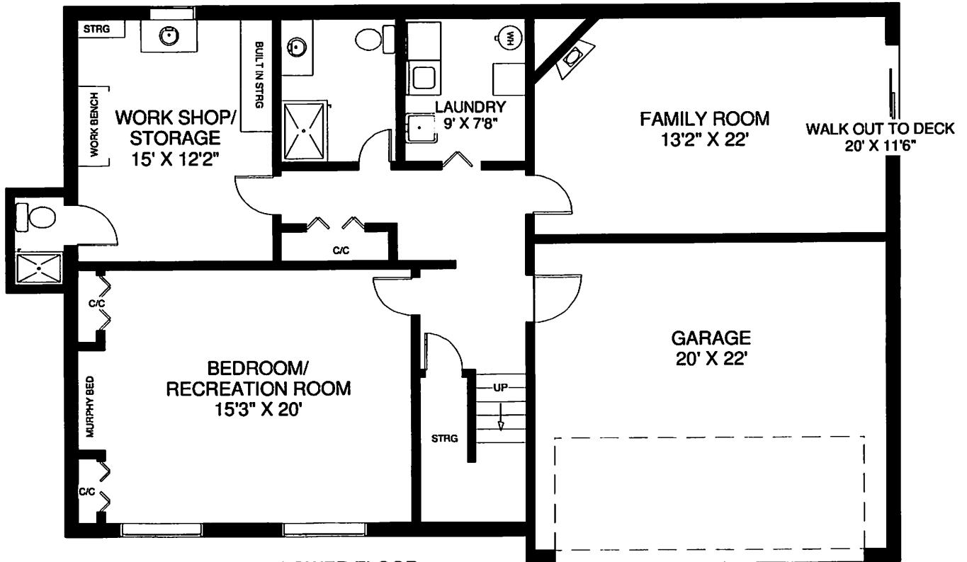
LOWER FLOOR APPROXIMATELY 1,340 SQ FT
