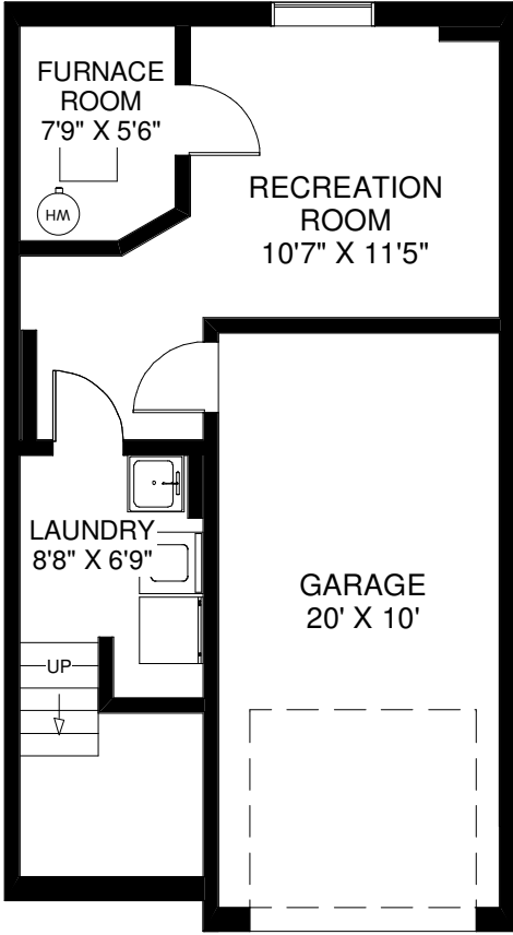
LOWER FLOOR APPROXIMATELY 370 SQ FT
