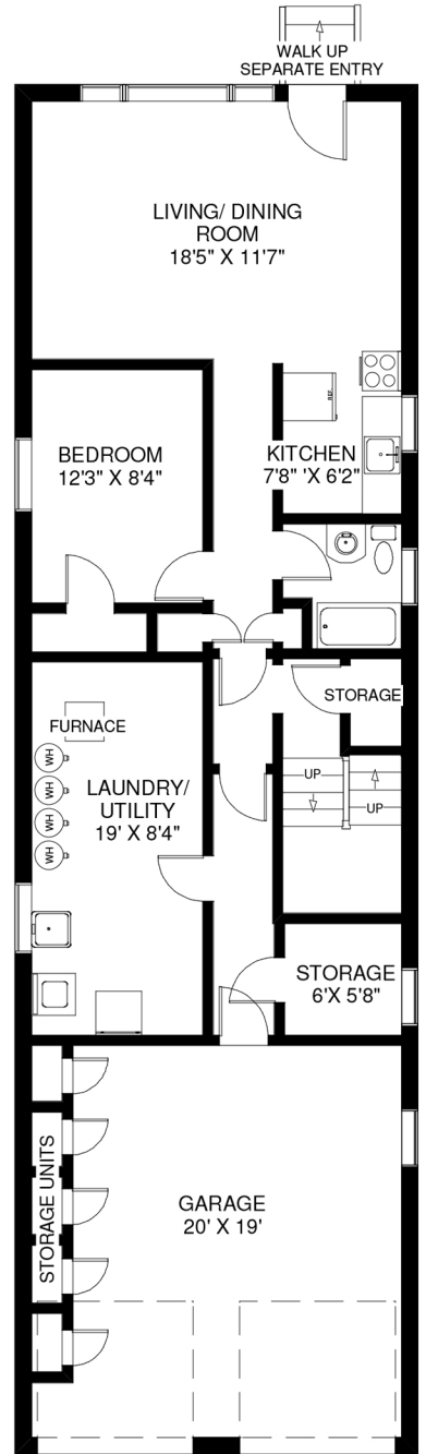
LOWER FLOOR APPROXIMATELY 1,025 SQ FT
