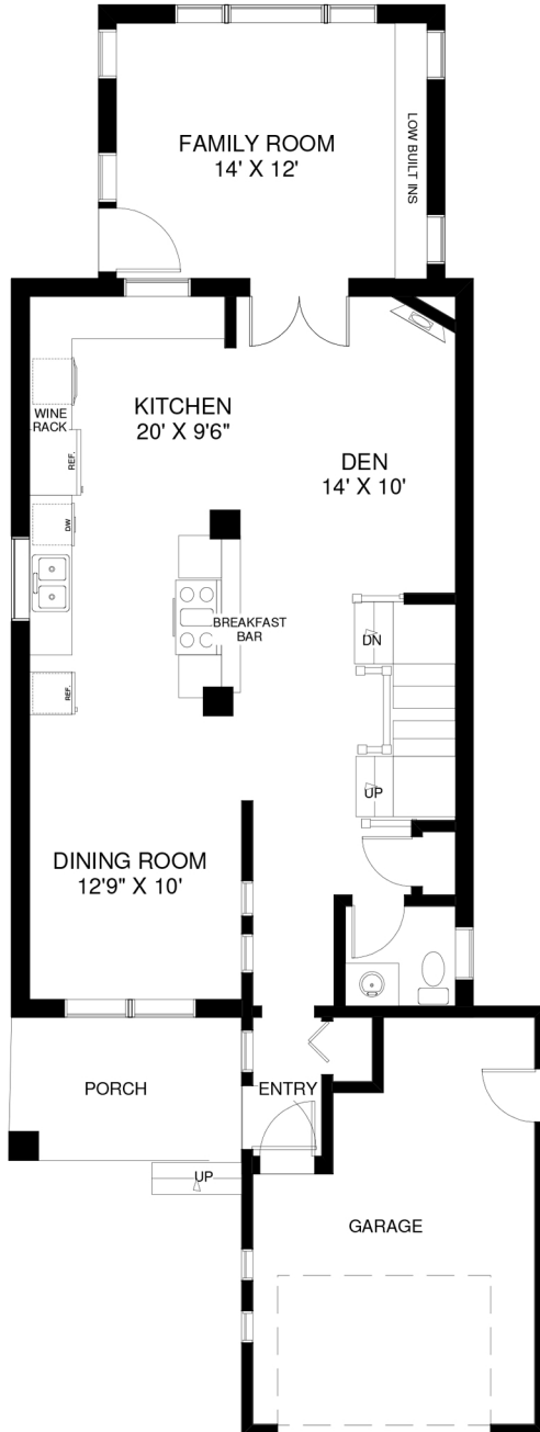
MAIN FLOOR APPROXIMATELY 1,000 SQ FT
