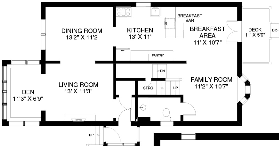
CEILING HT 8'6" MAIN FLOOR APPROXIMATELY 1,075 SQ FT
